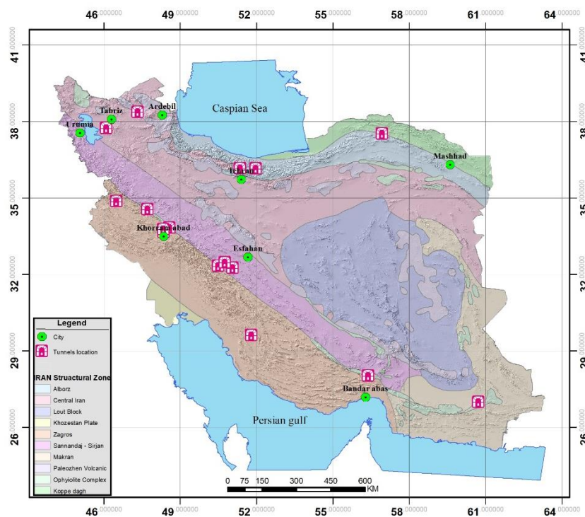
Fig. 1. Location of the studied tunnels on the structural zone map of Iran (Stöcklin,1968)
